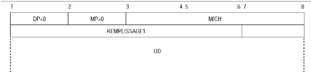
Figure 5-21. Paquet MSP COURT
