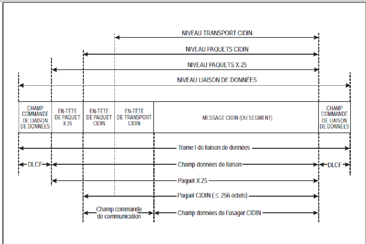
Figure 8-2. Terminologie CIDIN
