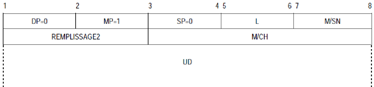
Figure 5-22. Paquet MSP LONG
